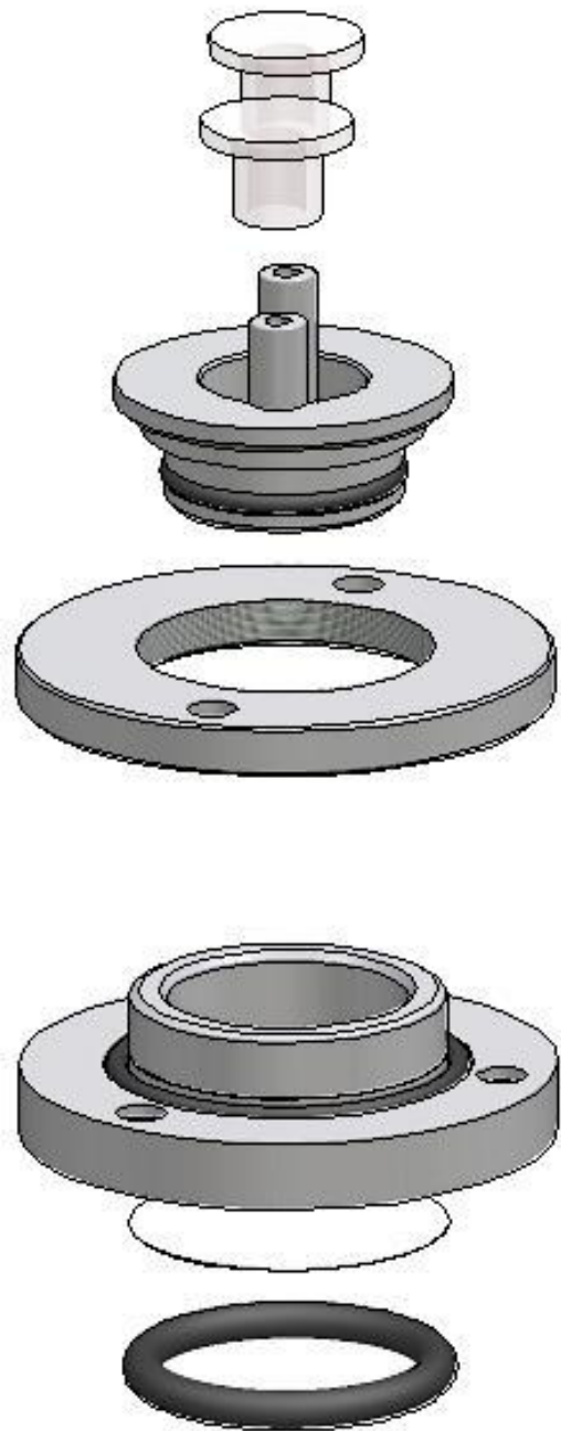
Mounting Nose for 3 Series Sensors
