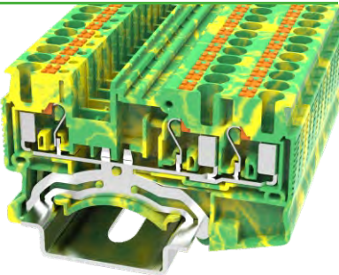
DS2.5-TW-PE
