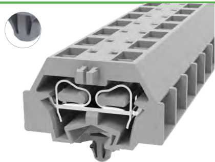
WS2.5T-DB-11A(H)
