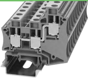
DC10-TW
