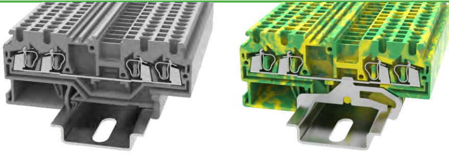
WS2.5-QU
