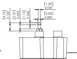
C- Barb Fitting Port B Only Configuration
