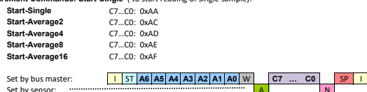
Figure 3 - I2C Communication Diagram
