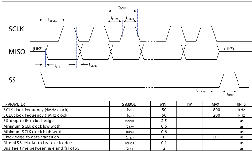
Figure 5 - SPI Timing Diagram
