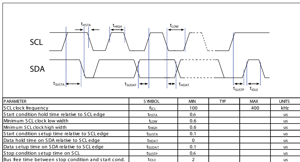
Figure 6 - I2C Timing Diagram
