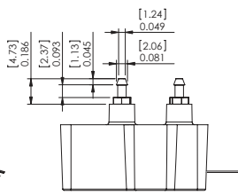
D- Barb Fitting Ports A and B Configuration
