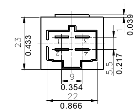
Mounting (Bottom view)
