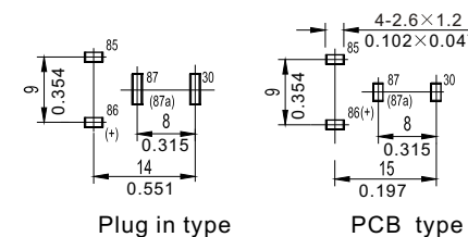
Plug in type PCB type Mounting (Bottom view)
