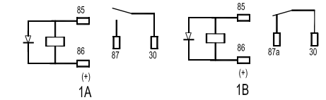
Wiring diagram (Bottom view)
