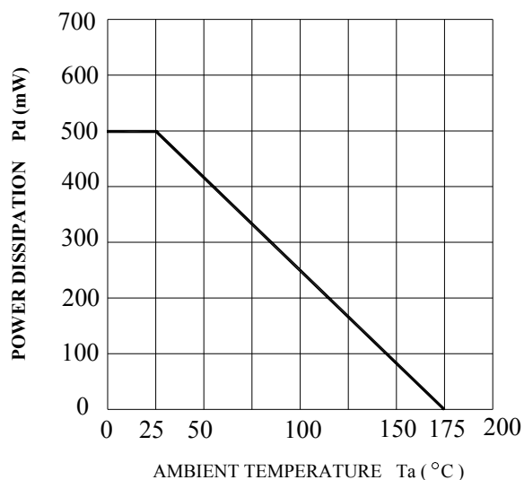
Fig. 2 Derating curve
