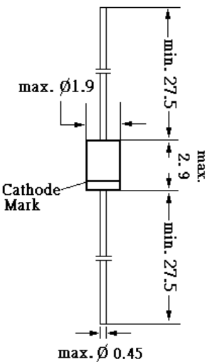
Glass case JEDEC DO-34 Dimensions in mm
