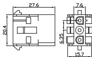
HOUSING WW210-F03
