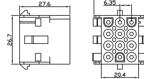
HOUSING WW210-F15
