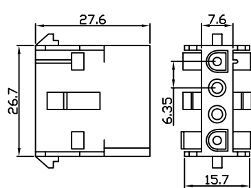
HOUSING WW210-F04
