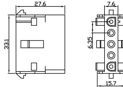
HOUSING WW210-F05
