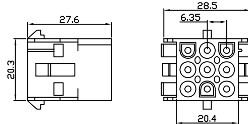
HOUSING WW210-F09
