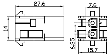
HOUSING WW210-F02
