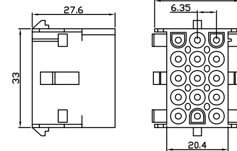
HOUSING WW210-F15
