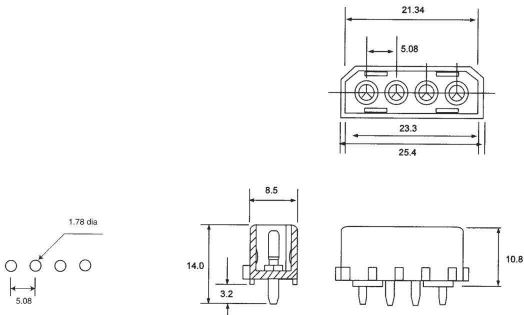
SPS2-R04 HEADER
