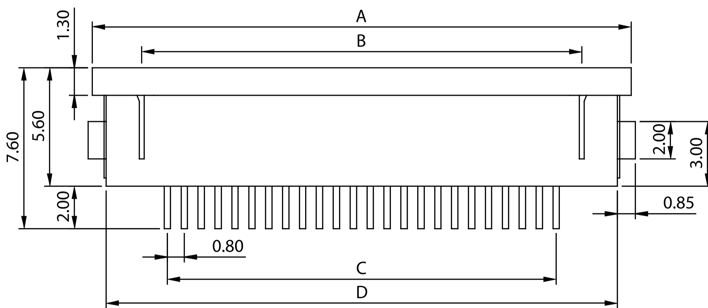
Bottom Contact
