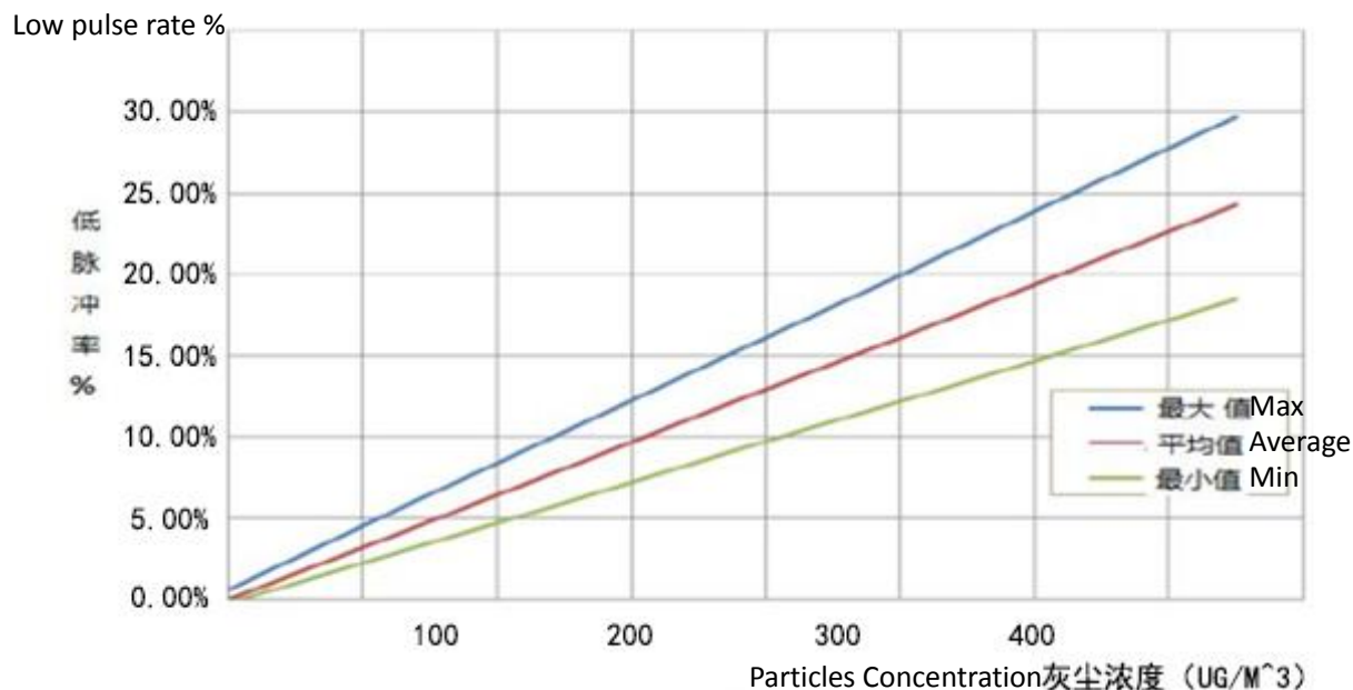
Fig9.The relationship of PM2.5 low pulse rate of output and dust particles concentration
