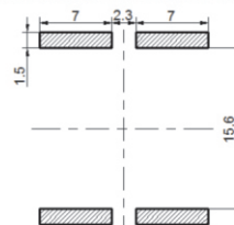
Recommended PCB Foot Pattern
